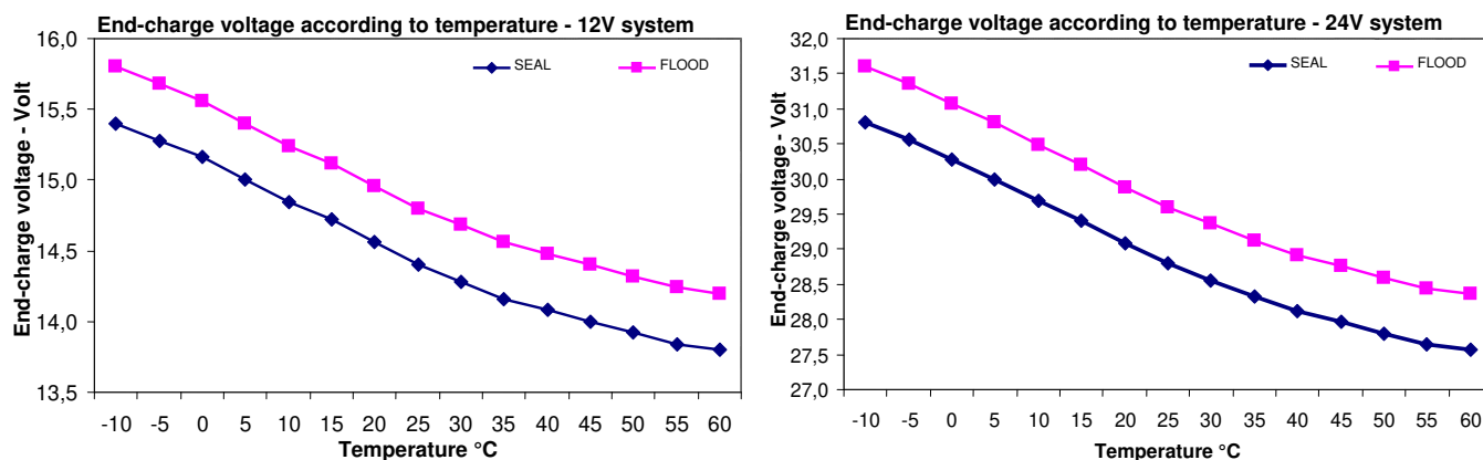
Pic.3 Compensation curve of Veoc charge voltage according to battery temperature
