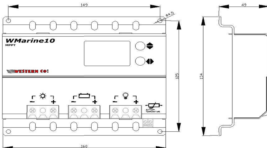
Fig.4 Dimensions
